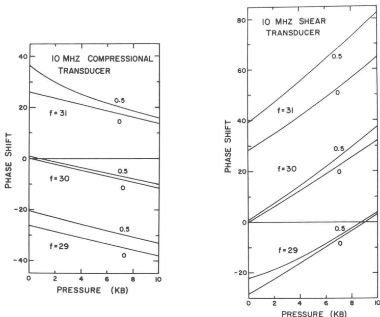
Fig. 6. (Left) Estimated effect of pressure on transducer-bond phase shifts for compressional [100] waves in \text{MgF}_2 with a 10-Mhz quartz transducer. Curves are for \tau_f = 0 and 0.5 nsec and carrier frequency f = 29, 30 , and 31 Mhz. Bond properties are estimated (Table 3). Fig. 7. (Right) As in Figure 6 for shear waves.
