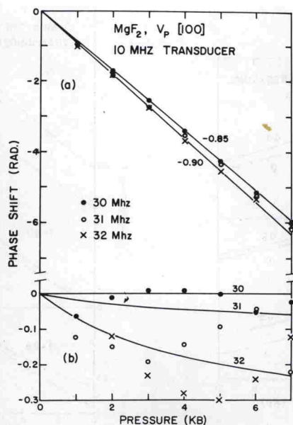
Fig. 8. (a) Measured phase shifts versus pressure (normalized to 30 Mhz) at 30, 31, and 32 Mhz for compressional [100] waves in \text{MgF}_2 . Lines are labelled with slopes (rad/kbar). (b) Residuals of measured phase shifts relative to line through 30 Mhz data, compared with calculated transducer bond phase shifts, assuming bond properties (Table 3) and \tau_f = 0.2 nsec.
